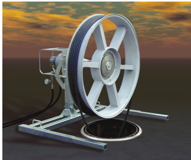
Hydraulically Limited Cable Puller with Mid-Assist Fiber Optic Capstan
