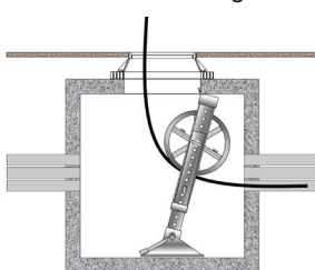
Jam Skid With Split Sheave Kit
