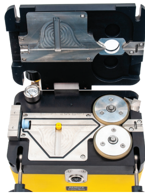
fitted with blowing plates for 1.7 to 5mm
