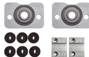
Cable Seal Collet Assemblies
