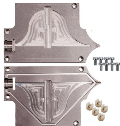
Buckle Plates
