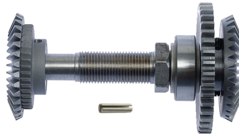
Rear Wheel Strand Drive - J2/C2 p/n 07558
