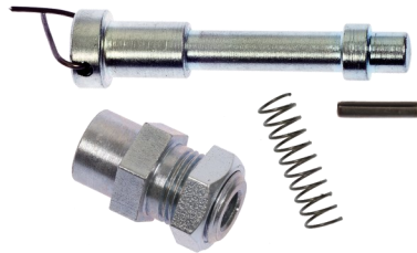
Plunger Kit - J2 p/n 33366
