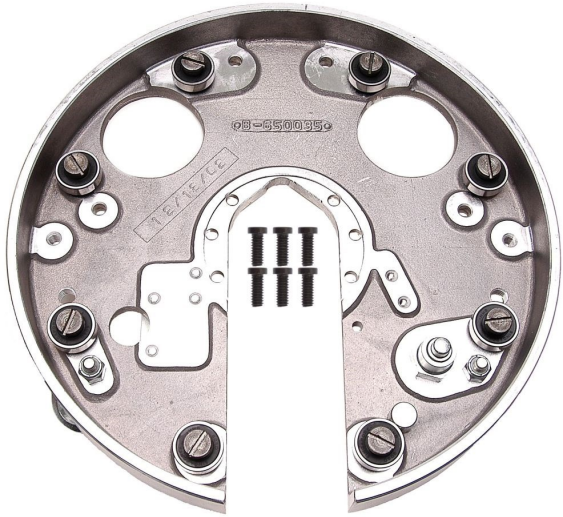
FRONT PLATE ASSY. - C2 p/n 27688
