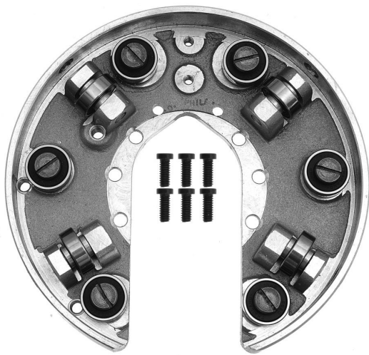
REAR PLATE ASSEMBLY - C2 p/n 27689
