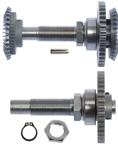
FRONT/REAR WHEEL STRAND DRIVE - J2/C2 p/n 35482
