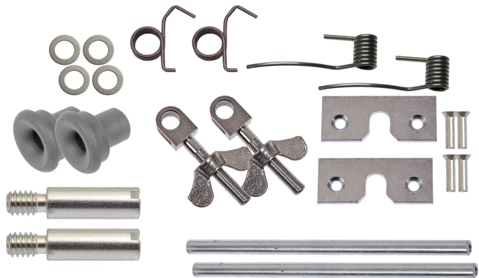
DOOR ACCESSORY KIT - C2 p/n 33407
