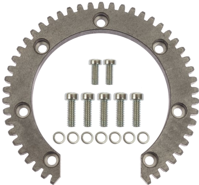
RING GEAR KIT - C2 p/n 33391
