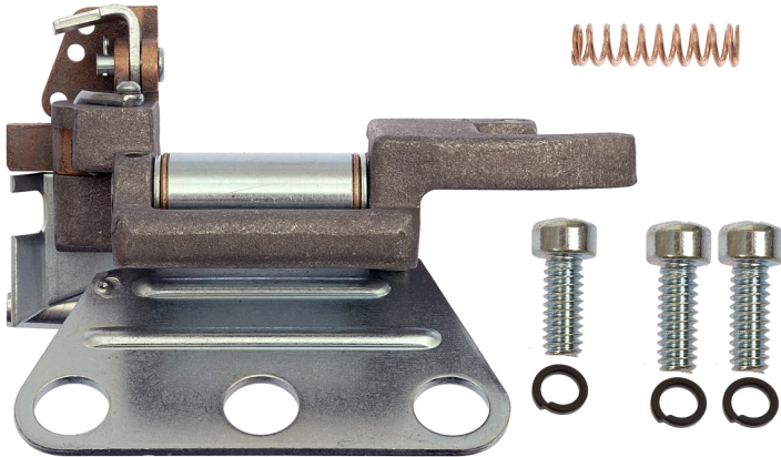
FRONT LIFTER ASSY COMPLETE. - C2 p/n 33397
