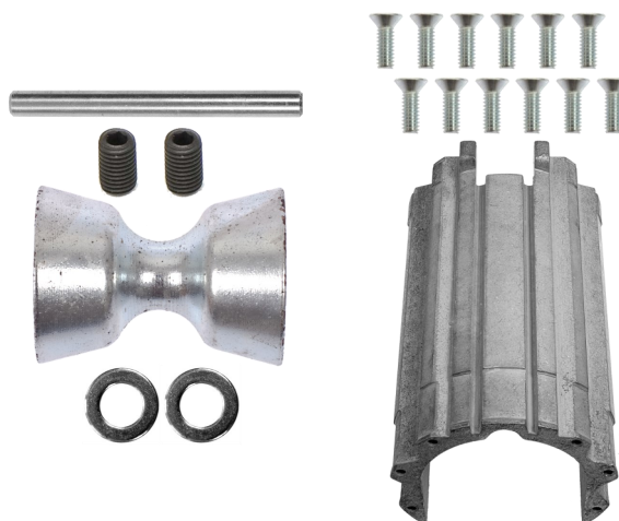
Trail Roller / Spacer Kit - J2 p/n 35485
