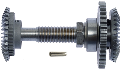
Gear Drive Housing Assy - J2B p/n 35512
