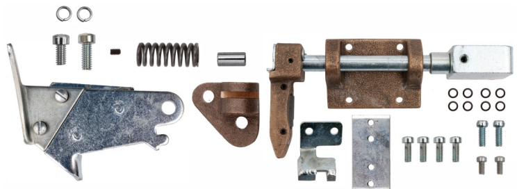
STRAND LOCK/PIVOT PLATE Kit - J LASHER ONLY p/n 35529
