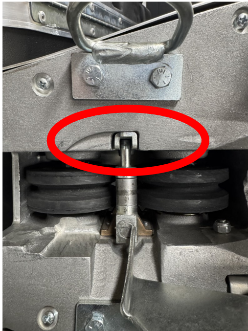
J2 HAS STRAND TENSION ROLLER GUIDE
