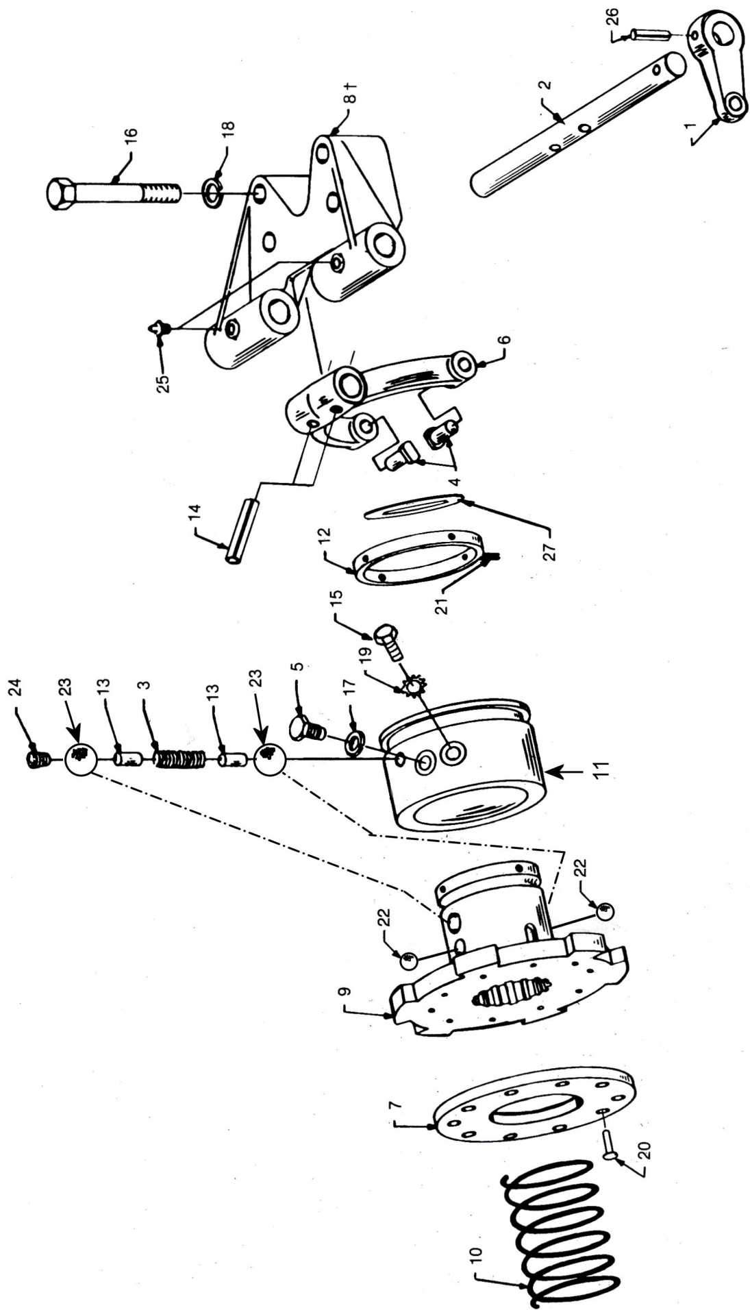
FIG. 5 — CLUTCH & DISC BRAKE ASSEMBLY PARTS DRAWING
