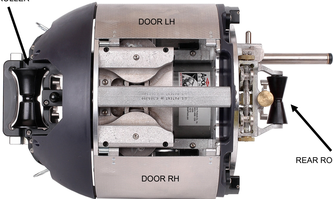
FRONT ROLLER
