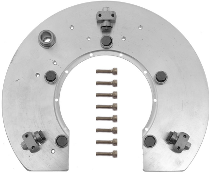
REAR PLATE ASSY - APOLLO p/n 33496
