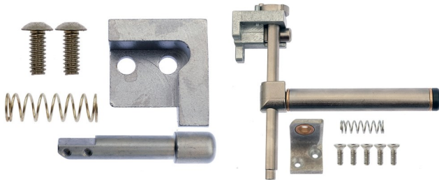
PLUNGER / REAR LIFTER KIT APOLLO p/n 35507
