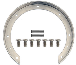
FRONT/ REAR BEARING RING KIT - 35499
