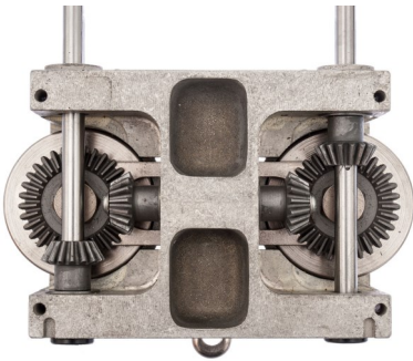
GEAR HOUSING ASSY - COMPLETE APOLLO p/n 27293
