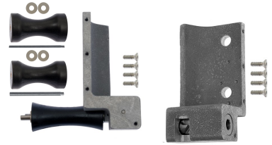
ITEM# 35498 R.H / L.H HOUSING KIT
