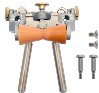
VERTICAL ASSY Kit APOLLO p/n 33511
