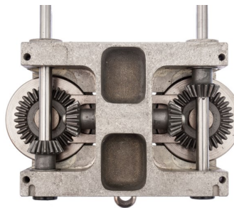
ITEM# 27293 GEAR HOUSING ASSY
