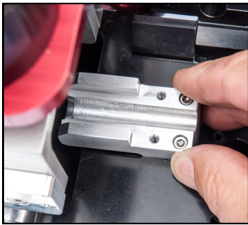
Place the guide in the groove on the exit side of the roller
